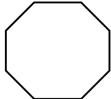
OCTAGON (8 sides)
