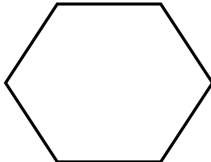
HEXAGON (6 sides)
